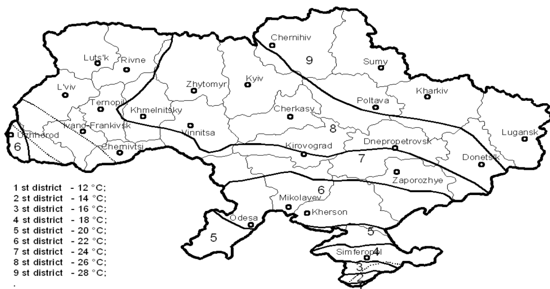
Figure 1. Zoning of Ukraine on the characteristic values of minimum air temperature X_0
