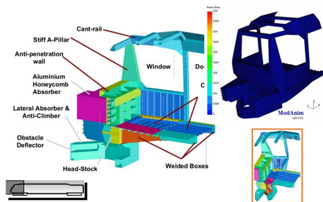
Figure 3. Computer modeling of the rolling stock
